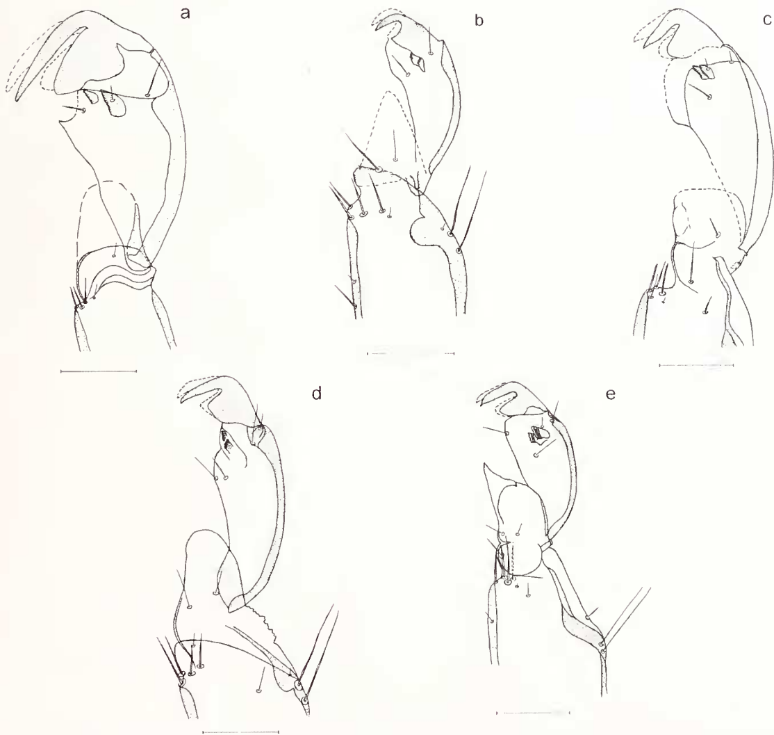
Fig. 7. Claws, two tarsal limbs and tip of tibia of a: Trochiloecetes ochotereui ?, b: Ricinus rubeculus , c: " Trochiliphagus ", d: R. dolichocephalus , and e: R. fringillae . Scale bar 0.1 mm.
